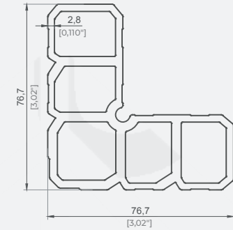
Cam Panel Köşe Takoğu Profili / Glass Panel Corner Block Profile
