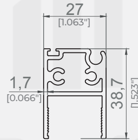
22mm Trabzan Profili / 22mm Handrail Profile
