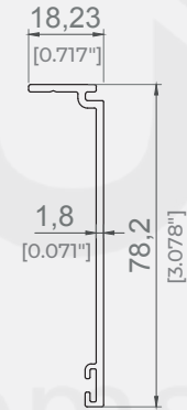
Yan Ray Kapak Profili / Side Rail Cover Profile
