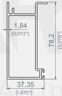
Yan Ray Dikme Profili / Side Rail Pillar Profile
