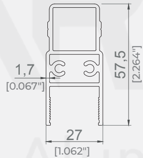
22mm Cam Panel Yan Profil / 22mm Glass Panel Side Profile
