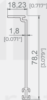
Yan Ray Orta Profil / Side Rail Middle Profile
